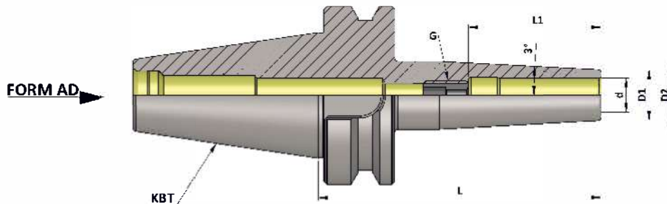
KBT (BT MAS 403) (SFH SLIM 3°) (AD) JD
